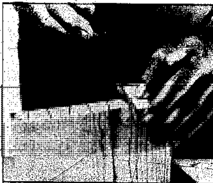
Use a template for marking and cuts when many dovetails are required.
