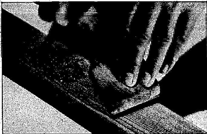
Hold scraper as shown and apply most of pressure with the hand over the blade. It is best to use a pulling stroke with this tool.
