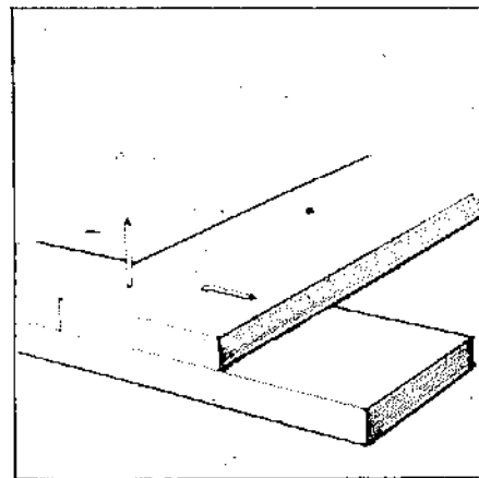
Nails may be clinched when appearance is not important. Be sure that the point of the bend is where the nail emerges. When clinching, you can back the head of the nail with another hammer if necessary.
