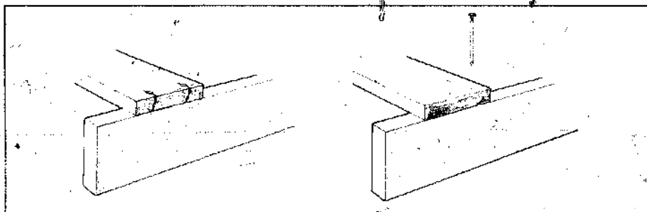
The wood can split when nails are driven close to an edge as shown on the left. In such situations its best to drill pilot holes first. Make the holes slightly smaller than the shank of the nail. Drill them through the piece to be fastened.
