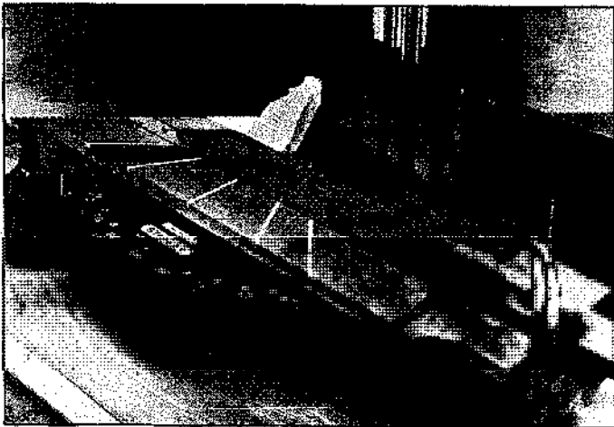
Compound-angle cuts are easy, even on covered molding, if you brace the work. The cut is then made as if it were a simple 45-degree miter.
