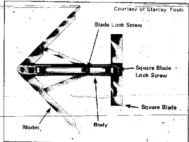
ANGLE DIVIDER for bisecting angles. The handle is graduated for marking angles for 4, 5, 6, 8 or 10-sided figures.
