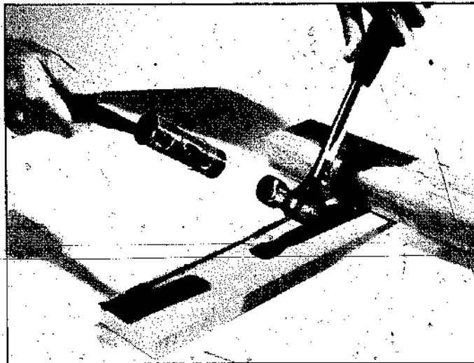
Use a soft-face mallet to drive ripping claws between pieces that must be pried apart. Never strike two steel hammerheads together.
