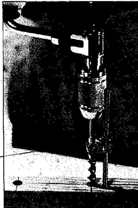
BIT GAUGE at left can control hole depth. It is attached by a clamp to the shank of the bit and can be used with any size cutter. The stop at right locks to the bit with a thumb screw.
