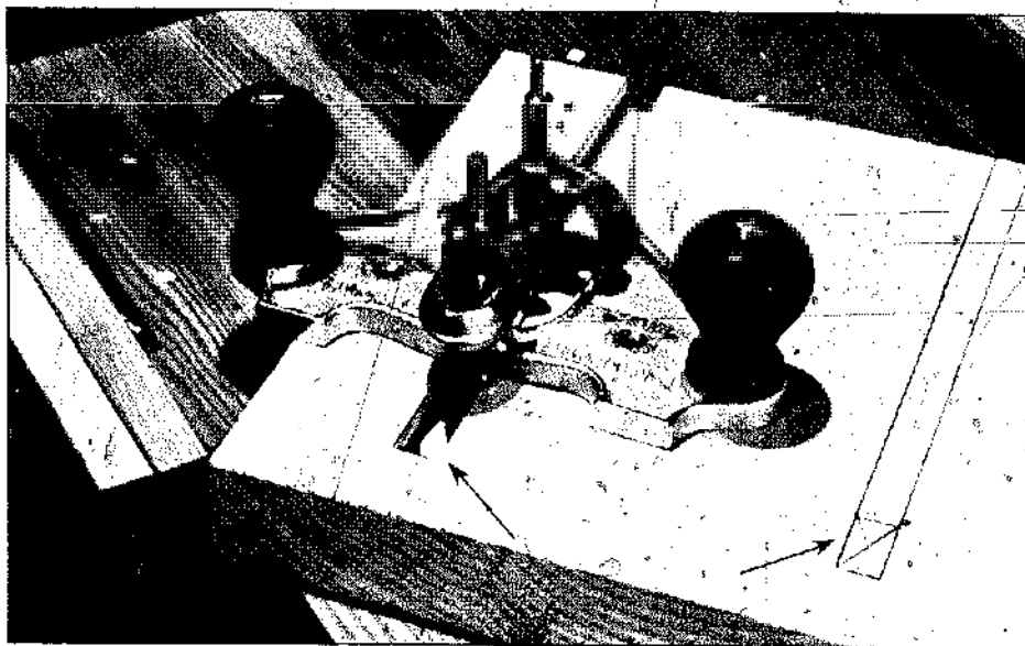
Arrows point out the part of a groove that must be cut with a chisel when a router plane is used to make a stopped cut.
