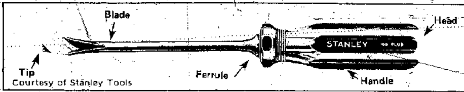
CONVENTIONAL SCREWDRIVER with wing-type blade.
