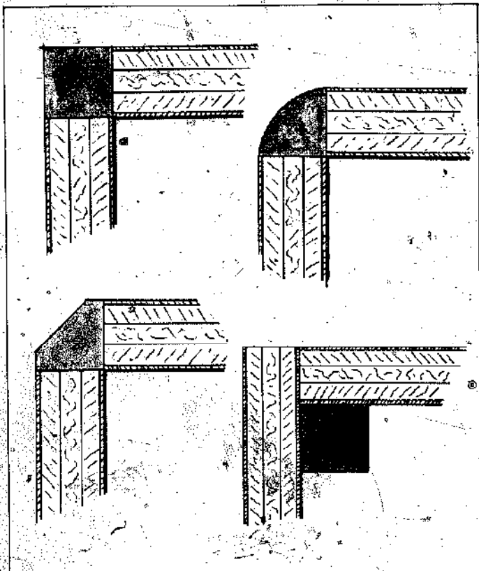
You can use solid-stock inserts to cover plywood edges at corners. They can be square, quarter-round, or triangular, and reinforced with glue blocks.
