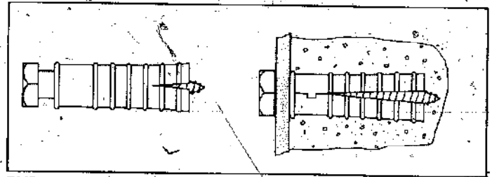
EXPANSION SHIELD
