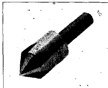
COUNTERSINK BITS , sometimes called rose head bits, are used to widen screwholes so the heads of flat-head screws will fit flush with, or slightly below the surface of the work. Properly tempered, they may be used with soft metals such as aluminum or brass.
