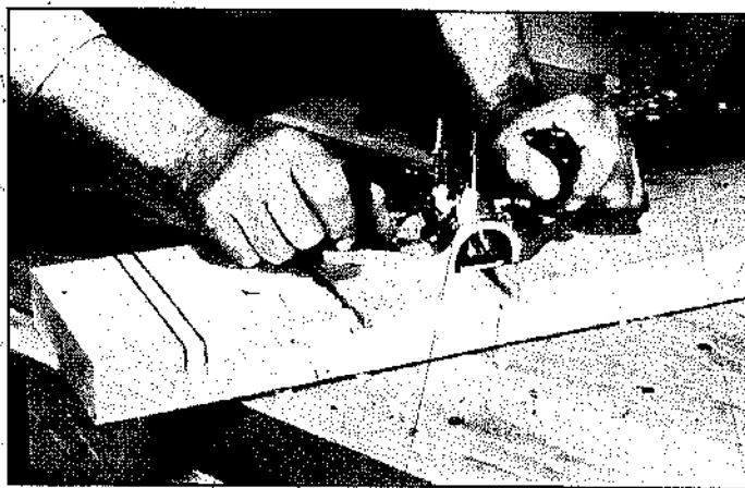
ROUTER PLANES can be used to finish a dado. The job should be started by making shoulder cuts with a saw as shown at left.
