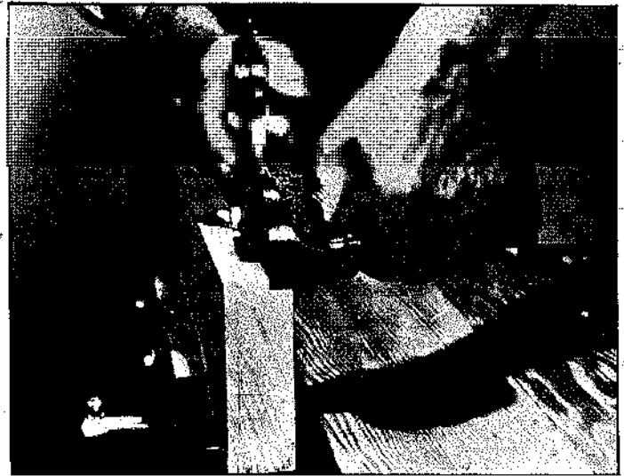
Set your RABBIT PLANE to the proper depth and width for an L-shaped cut. Be sure to make all passes with the fence snug against the side of the work.
