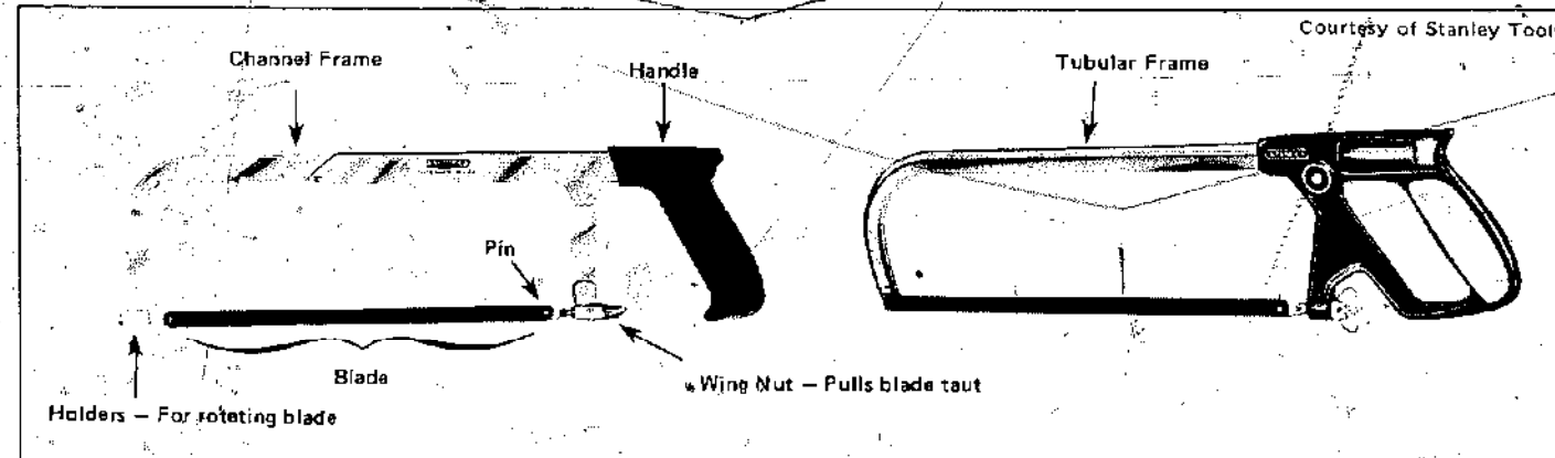
HACKSAWS are made with two types of frames: CHANNEL-FRAME and TUBULAR FRAME. Both are adjustable.
