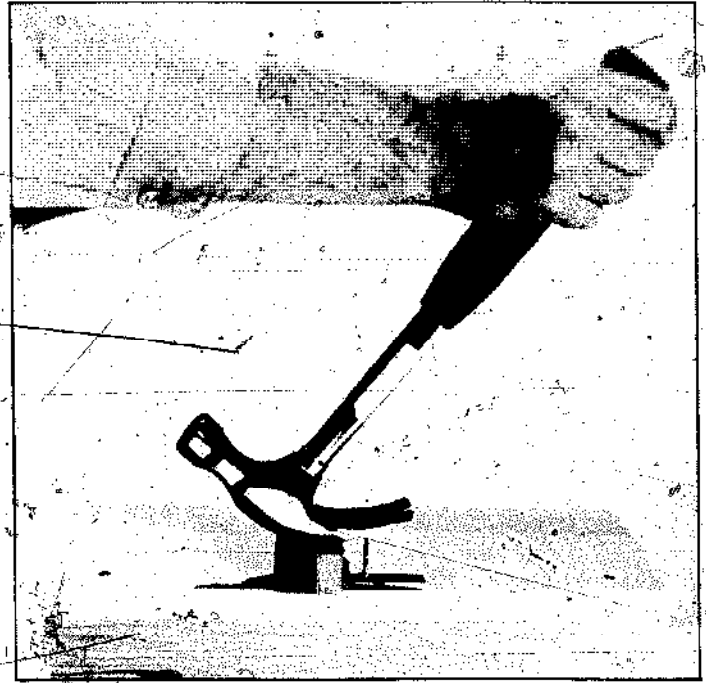
A block of scrap wood placed under the hammerhead increases leverage tremendously. The nail is removed easily and the hammer is protected from undue stress.
