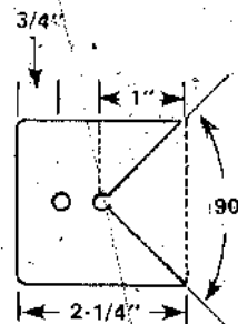
Countersink the underside of each hole for a 1/4-inch flat-head machine screw.
