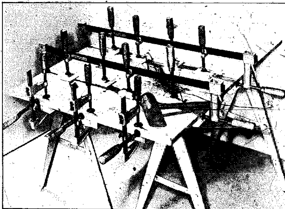
BAR CLAMPS are used here with edge clamps to apply pressure downward on the work as well as against its sides.
