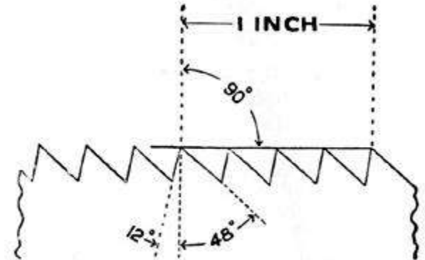
Angles of crosscut teeth 1/4 inch space or five points to inch.
