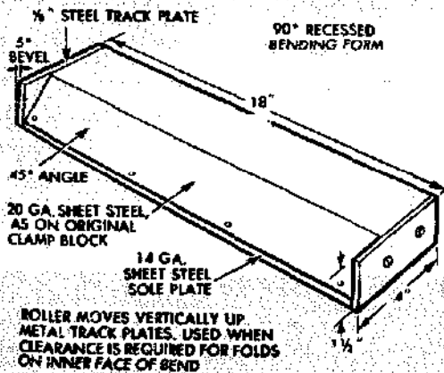
RECESSED FORM is a versatile accessory. It can be used to construct boxes and bend narrow channels
