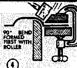
④ 90° BEND FORMED FIRST WITH ROLLER REVERSE RADIUS BEND USING MOLD AND Mallet
