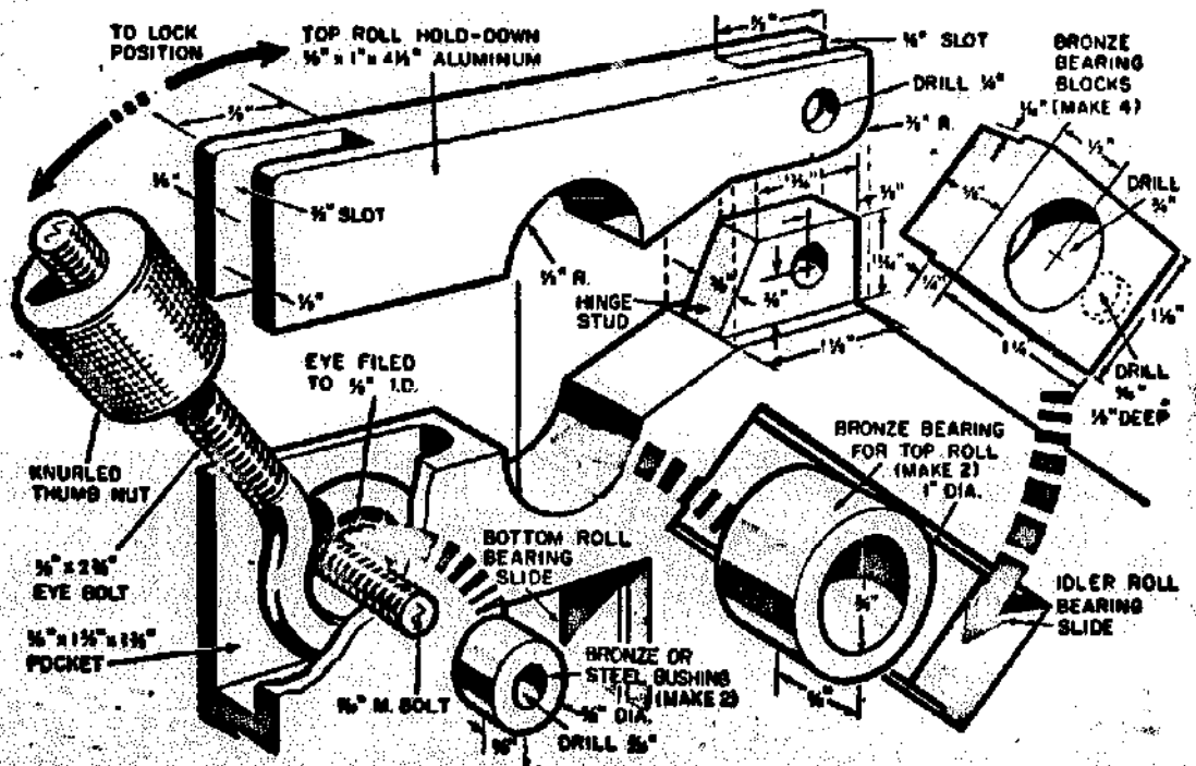
WHEN MILLING POCKET, avoid chatter by feeding work in .0005-in. steps and dropping cutter like a drill
