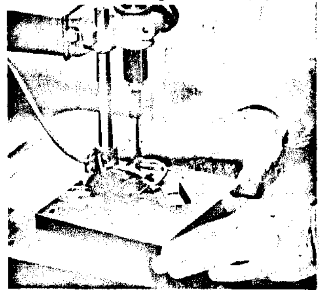
REMOVING FORMED CYLINDER is simple matter of unlocking top roll and lifting one end to slip cylinder free. Note base is clamped (or permanently bolted) to bench to handle overhangs and for clearance
