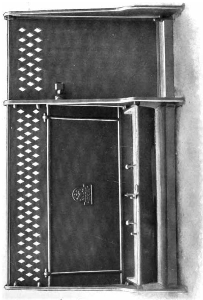
Fig. 141. —Iron Fittings for Picgeries (Musgrave). In the figure the swing flap over the trough is pushed back, thus cutting it off from the sty.
