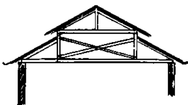
Fig. 85.—Open Roof.
