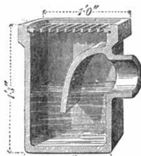
Fig. 166.—A Gully Trap.
