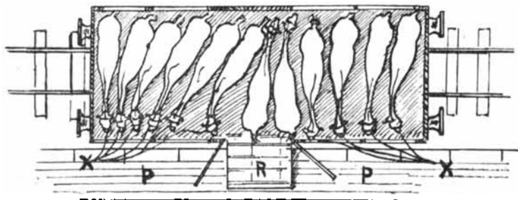
Fig. 214.—Diagram of truck loaded with horses. PP is the platform; R, the ramp leading into the truck. At XX stands a man to receive the head-ropes as the horses are loaded.
