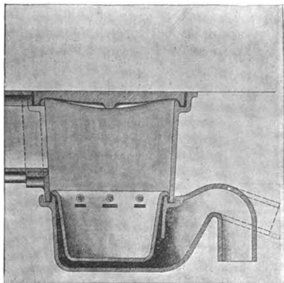
Fig. 184.—Fixed Syphon Stable Trap with removable bucket.
