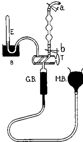
FIG. 203.—Diagram of one Form of Mercury Pump for Collecting the Gases of the Blood. M.B. , the mercury bulb which can be raised so as to fill G.B. and a-b with mercury, and lowered so as to produce a Torricellian vacuum in them. a and b , clamps by which the blood bulbs may be shut off, to be weighed and to receive the blood. G.B. , the bulb in which the gases are collected. T. , the three-way tap by which the gas bulb G.B. is connected, either with the blood bulb, or with the eudiometer tube, E. B. is the bath of mercury in which the tube filled with mercury is set.
