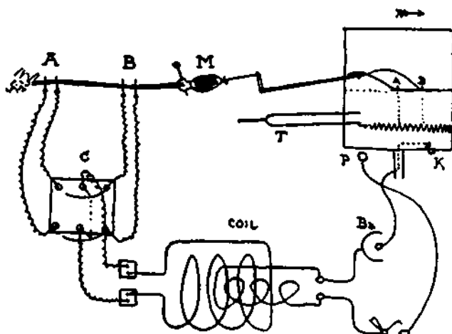
FIG. 30.— M , Muscle attached to crank lever marking on revolving drum. The secondary circuit of an induction coil is connected with a commutator, with the crossed wires removed so that the current may be sent either through the wires going to the nerve at A far from the muscle, or at B , a point at a measured distance nearer the muscle. On the drum, A represents the onset of contraction on stimulating at A , and B the onset on stimulating at B . To secure stimulation in each case with the drum in the same position, the make and break of the primary circuit is caused by the point of K touching and quitting the point P .
