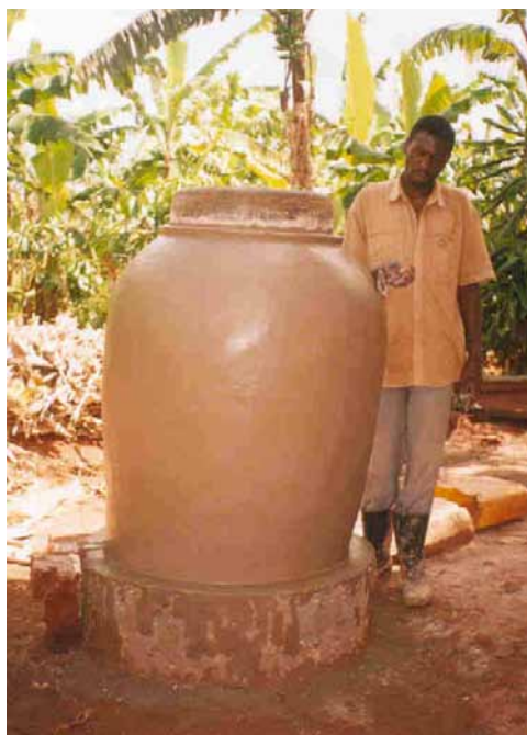
Figure 9 - 400 litre water storage jars being constructed as part of the water quality testing experiments in Uganda
