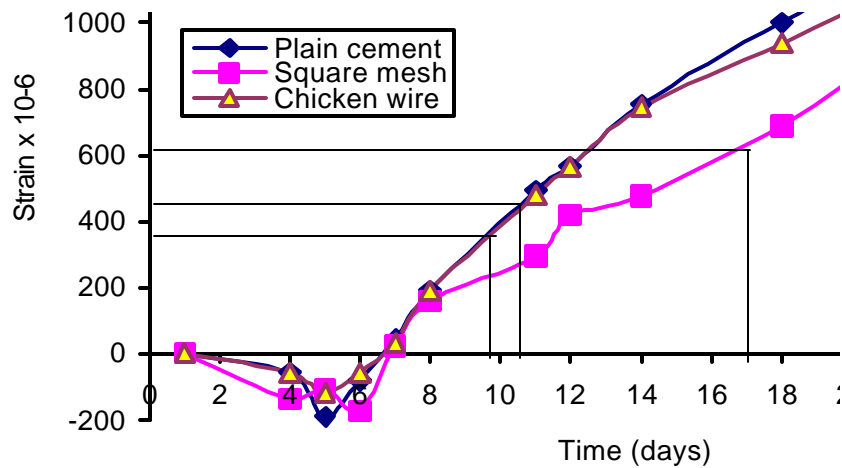
Fig 5.12 Breaking strain
