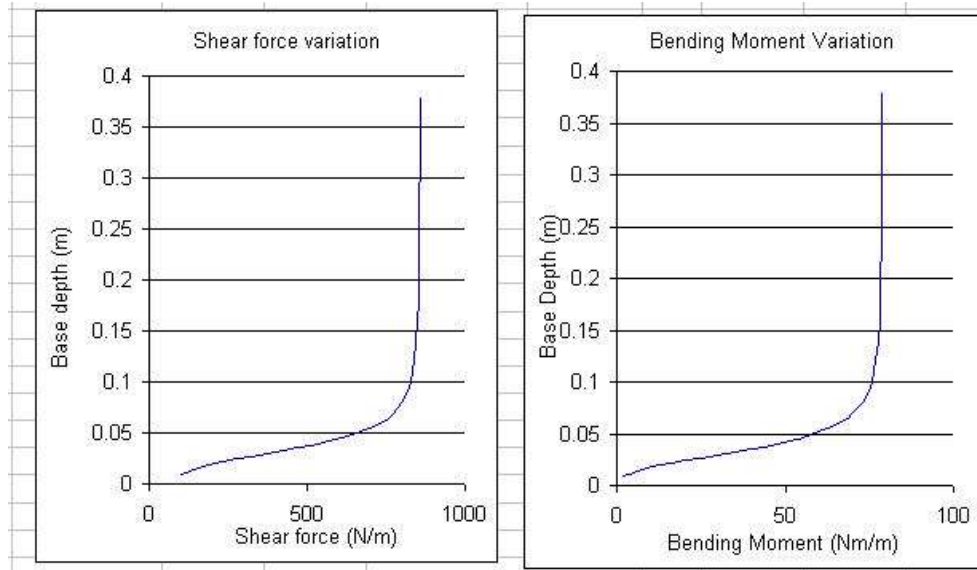
Fig. 2.12 Variation in shear force and bending moment
