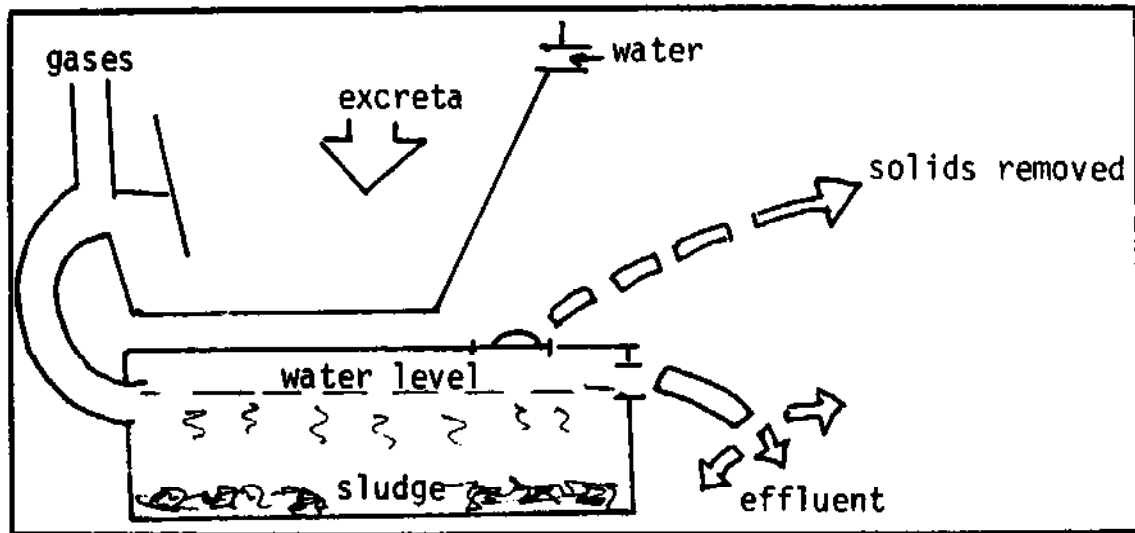
Figure 20. Septic System
