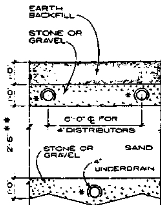
SECTION - BED TYPE
