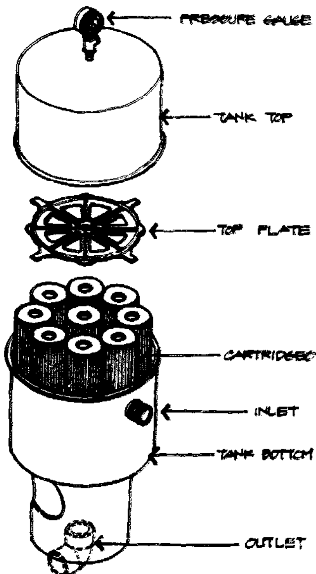
CARTRIDGE FILTER SYSTEM CLEANABLE POLYESTER FIBER TYPE
