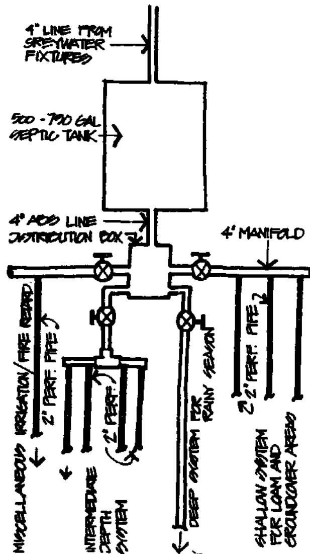
MORRISON, JACONI SYSTEM DIAGRAM
