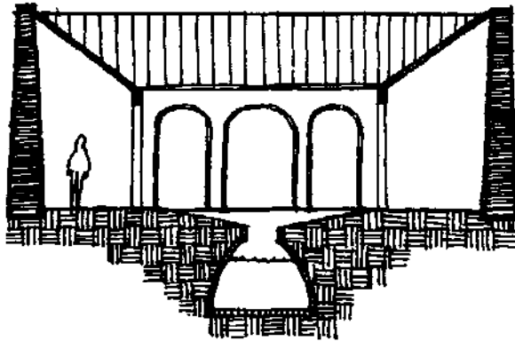
TRADITIONAL ATRIUM-TYPE HOUSE DESIGNED TO COLLECT RAINWATER
