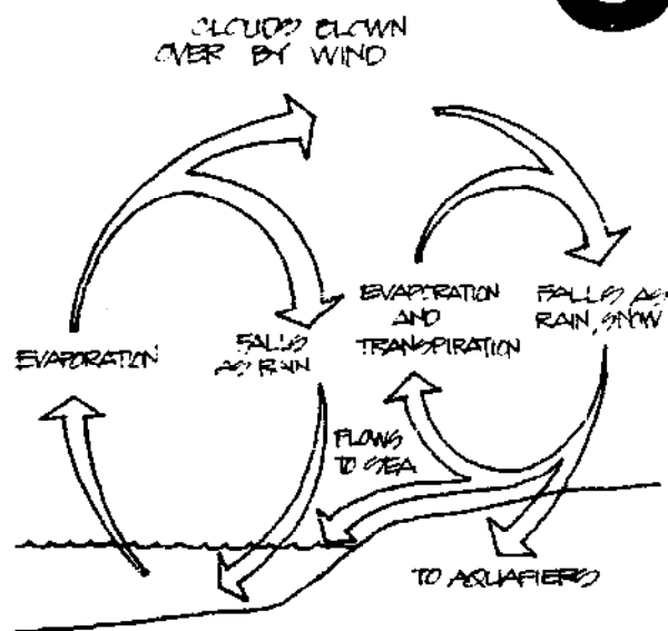
HYDROLOGIC CYCLE
