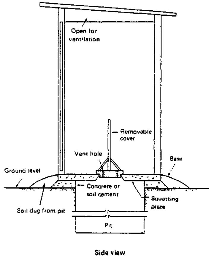
Figure 5 - Section of a Pit Latrine (millimeters)
