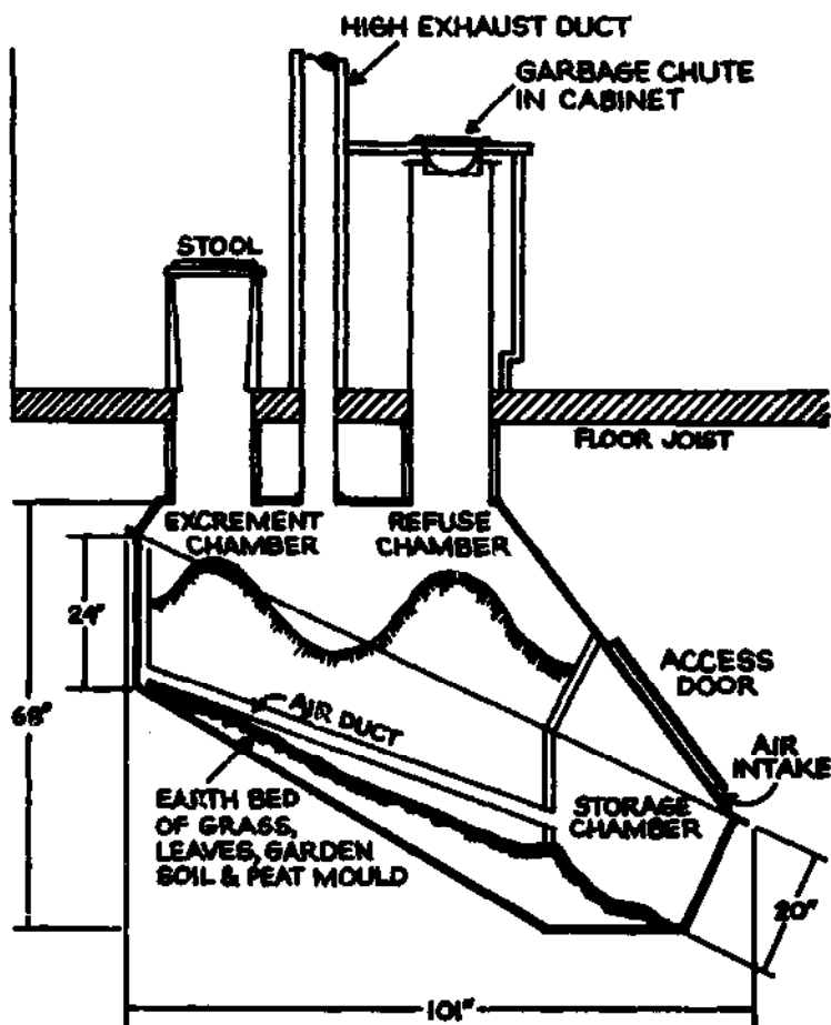
Cross section of the Clivus Multrum
