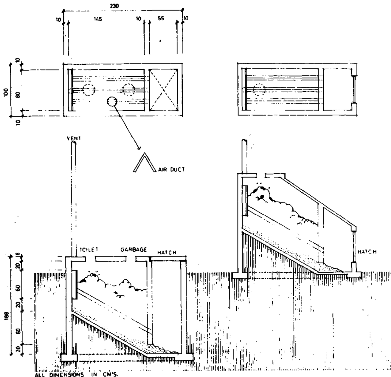
The Minimus composting toilet (from 2224).
