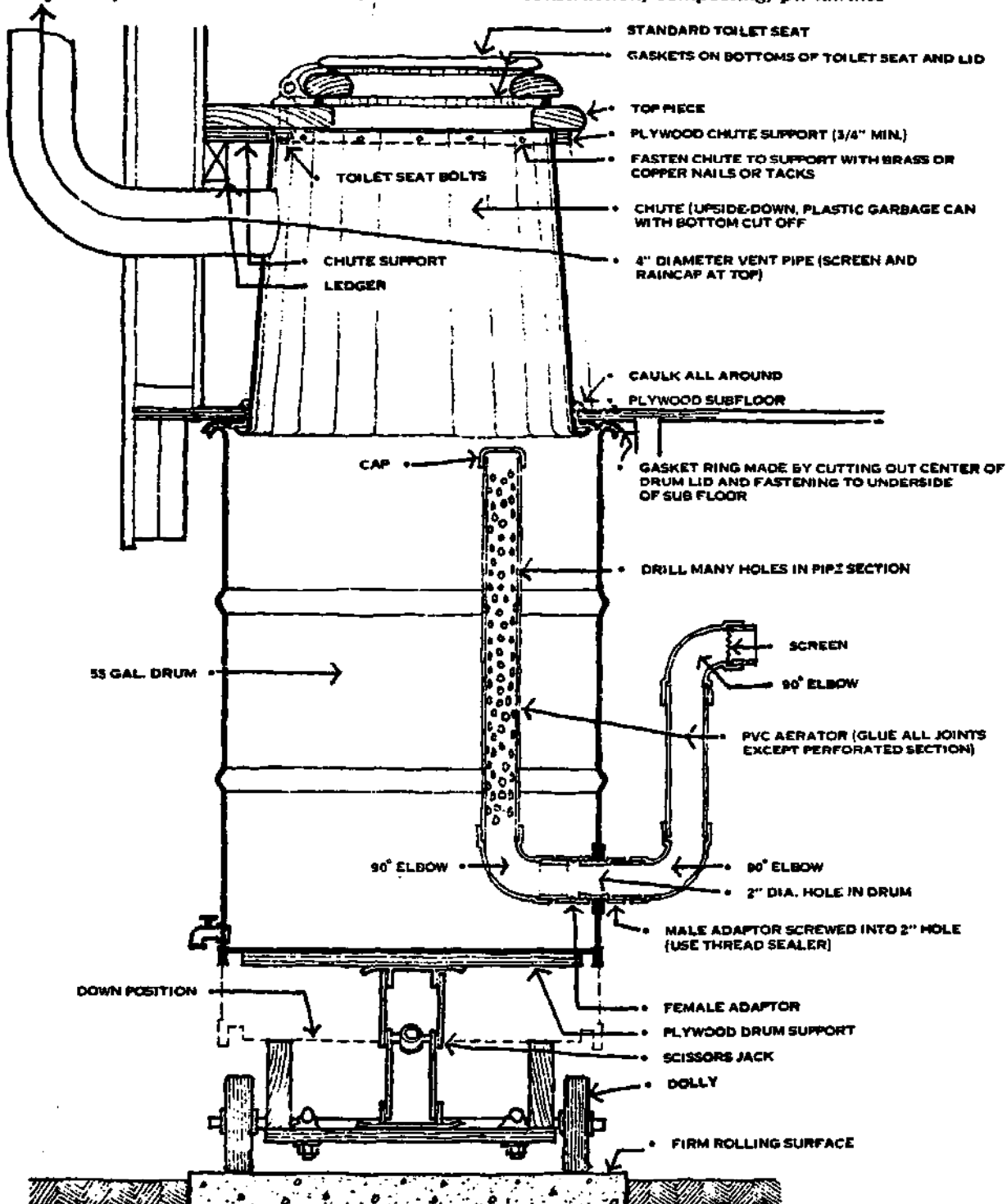
Matson drum privy (from 2135).
