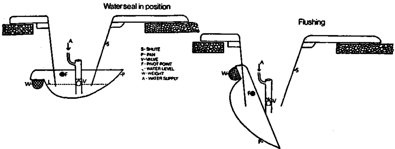
The Watergate flushing pan (from 1008).
