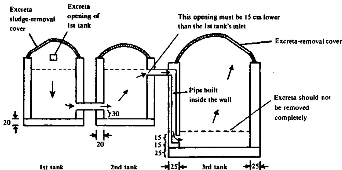
The Chinese three-tank toilet (from 2303).
