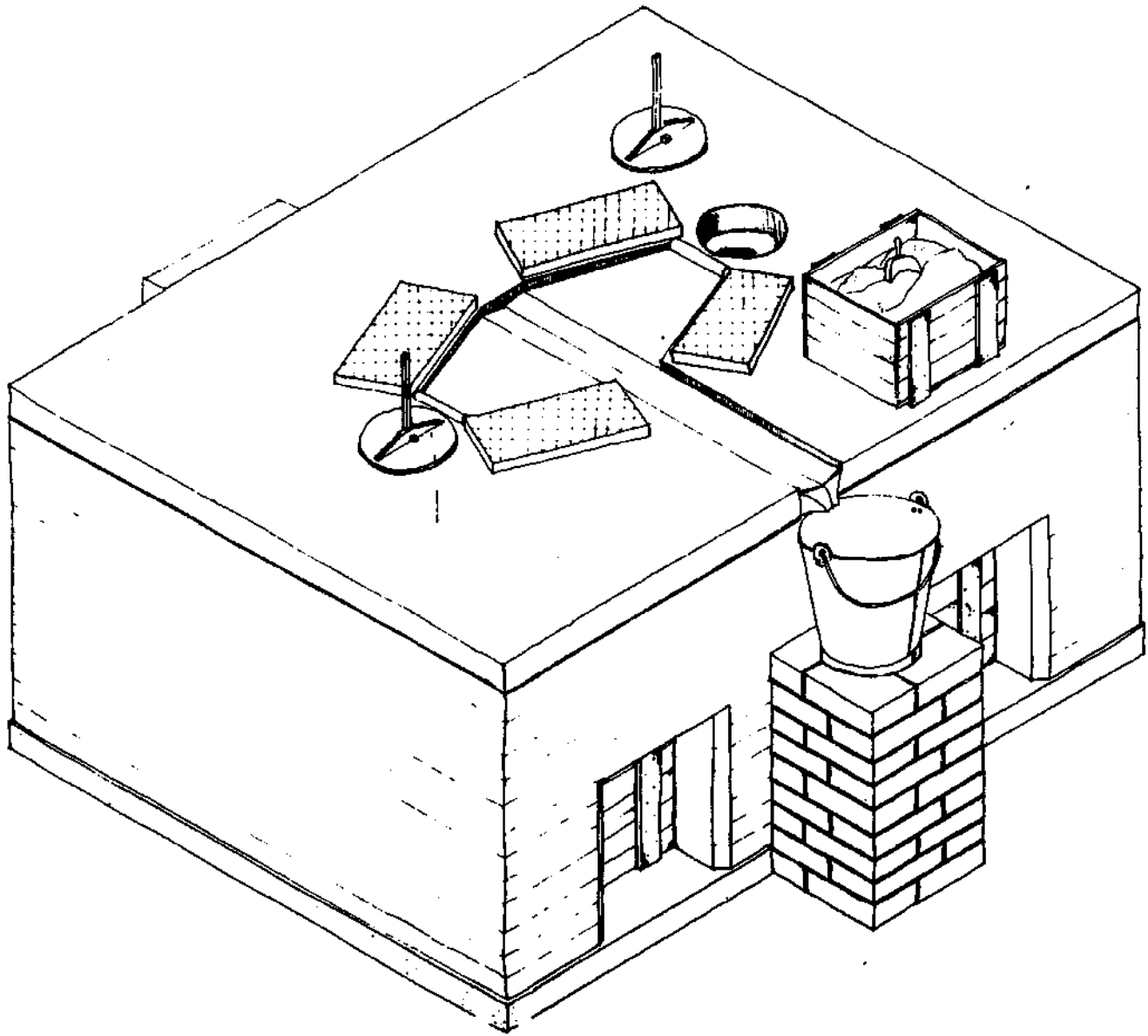
The Vietnamese double vault.
