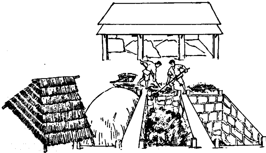
Full pit covered with earth and sheltered
