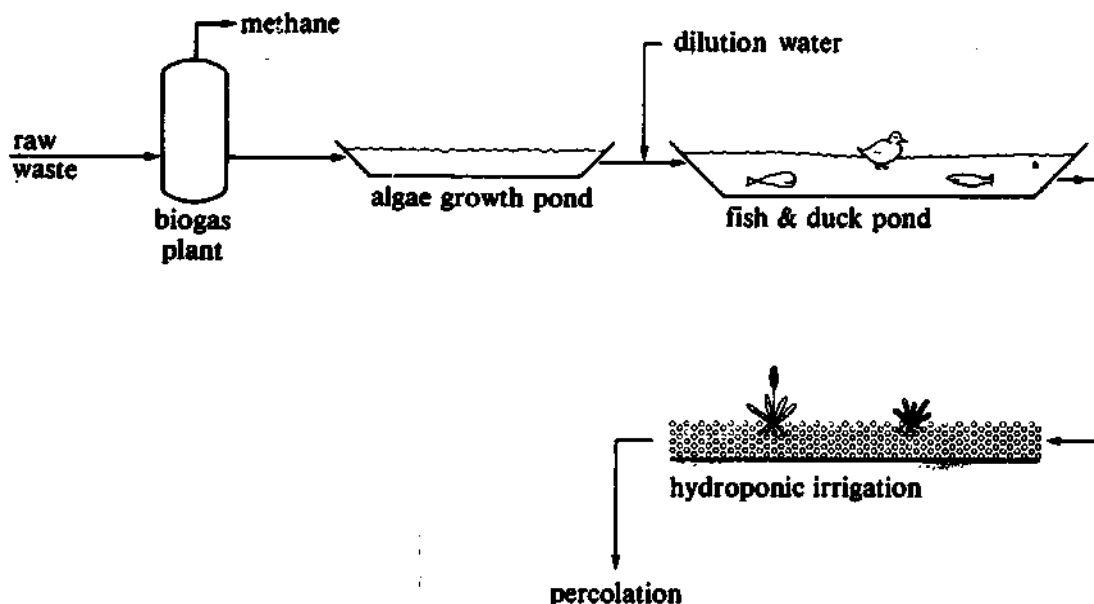
Integrated waste-disposal system (from 4509).
