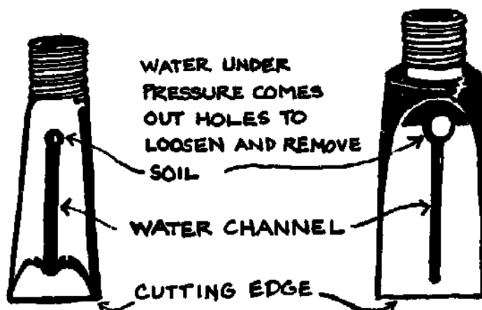
FIG. 14-12. JETTING BITS
