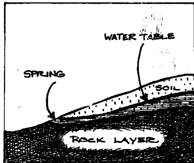
FIG. 1-1. SPRING LOCATION
