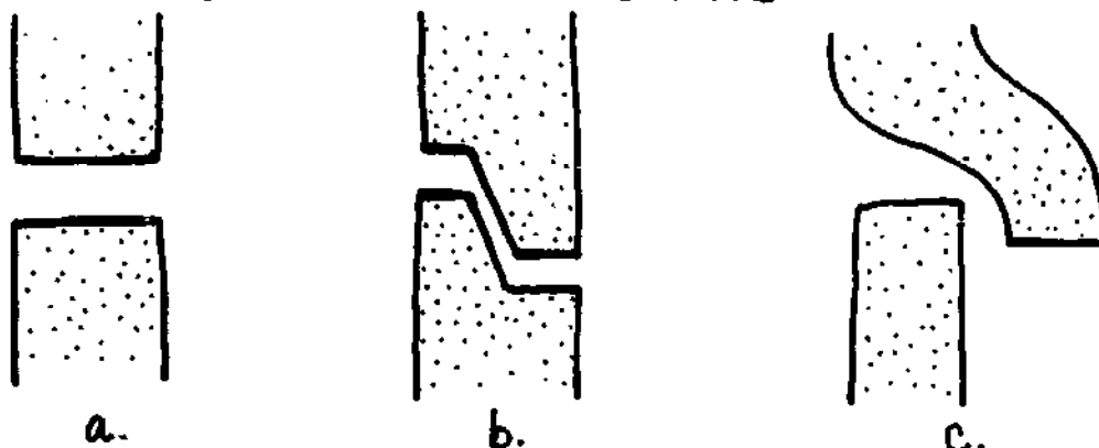
FIG. 8-8. CONCRETE LINING RING JOINTS
