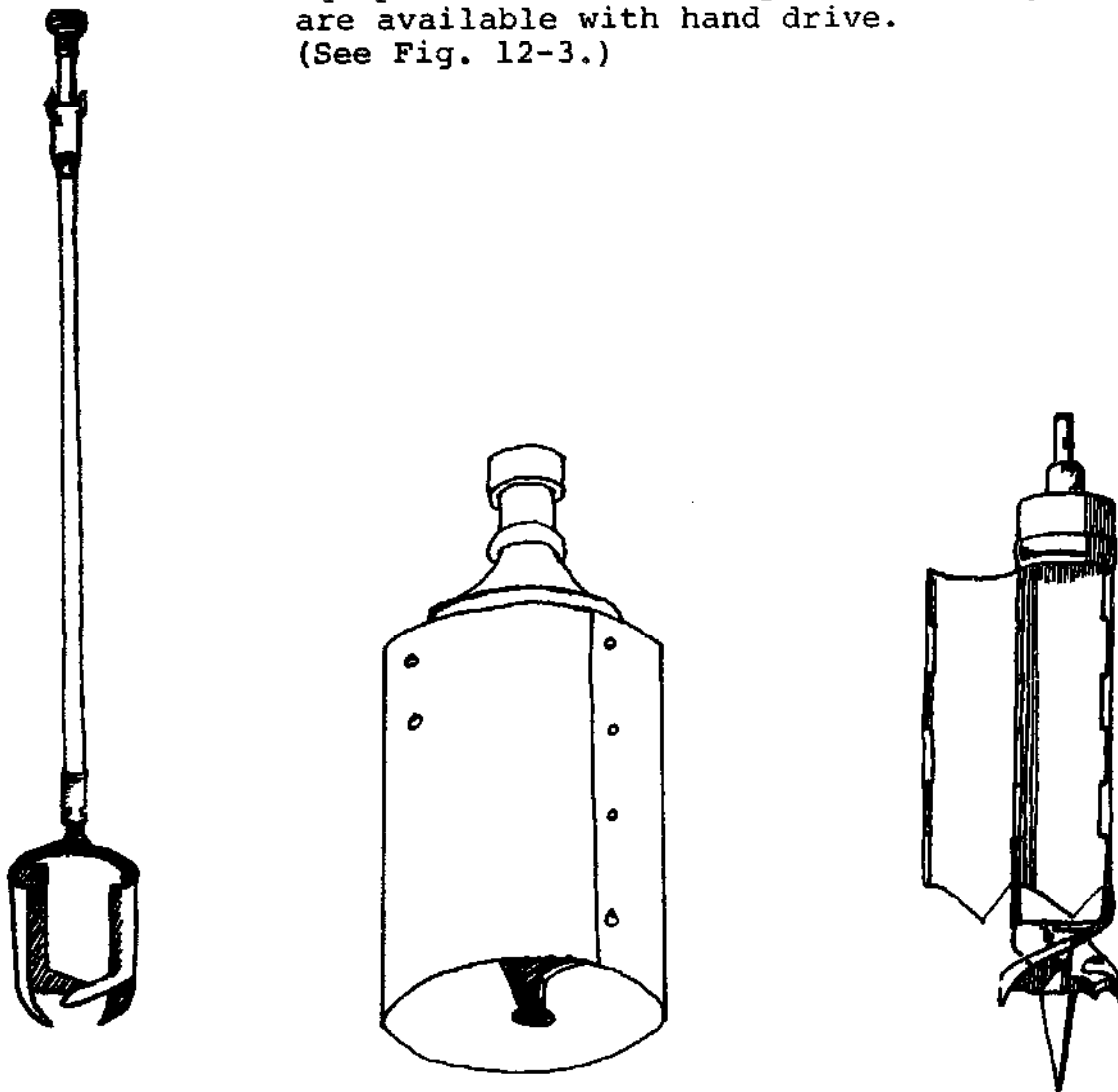
FIG.12-2. BUCKET AUGERS
