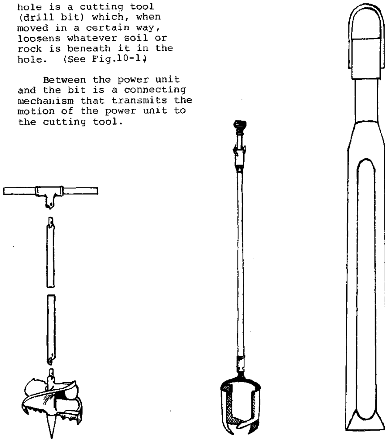
FIG. 10-1. DRILL BITS
