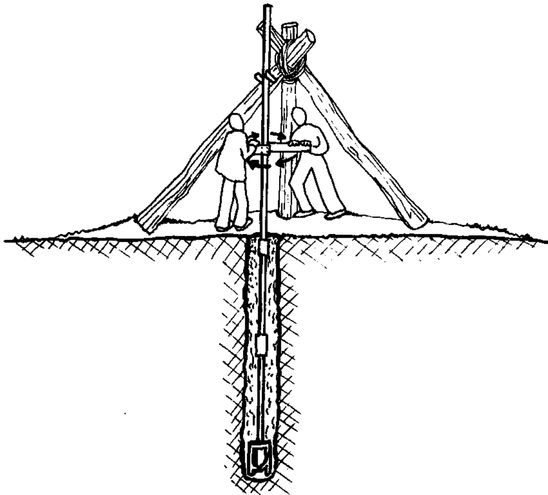
FIG. 11-3. HAND AUGERING
