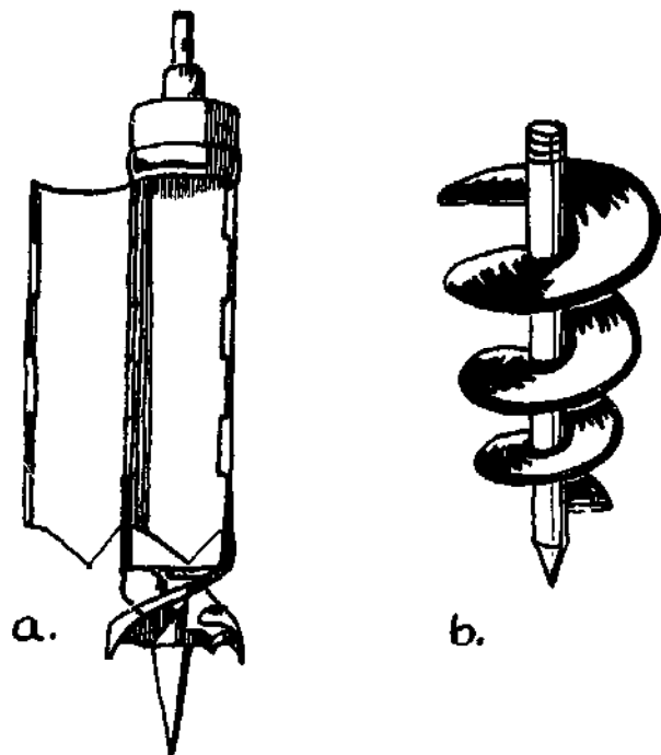
FIG. 10-4. AUGER BITS.
