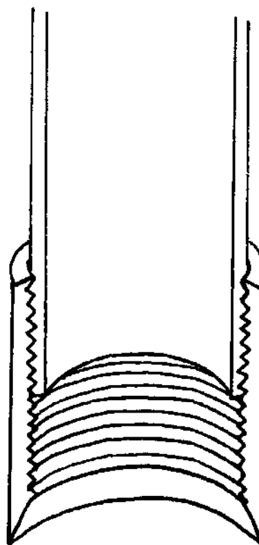
FIG. 13-2. SHARPENED COUPLING
