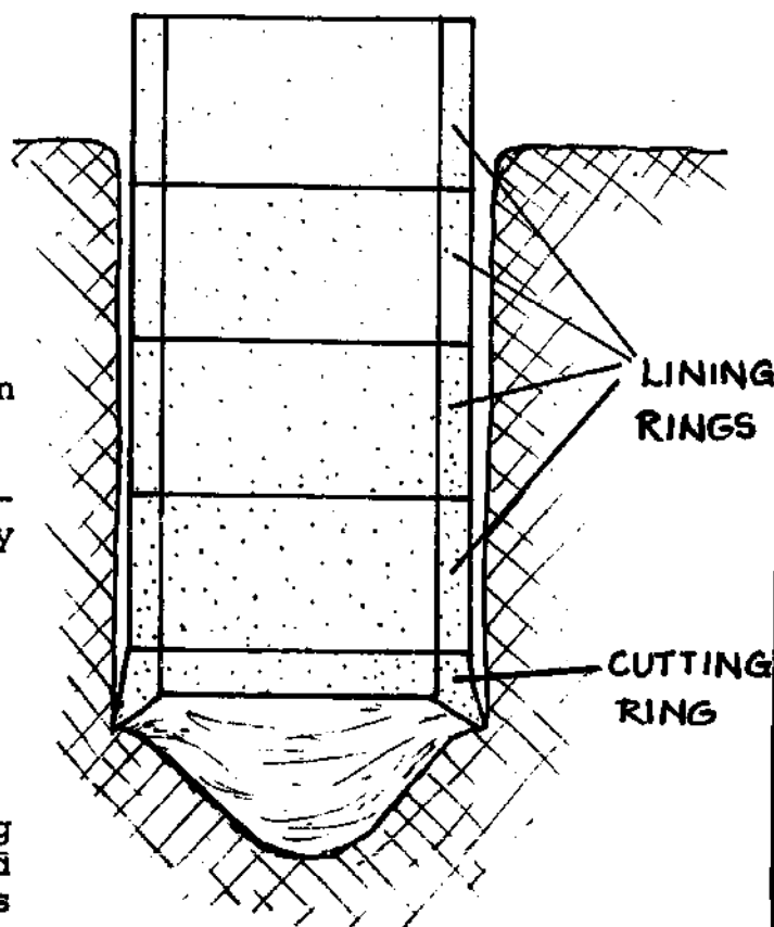
FIG. 7-1. SINK LINING
