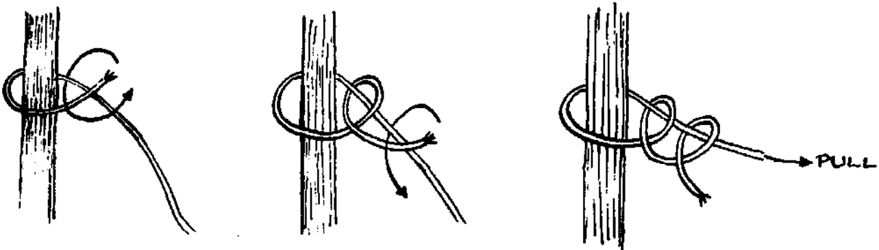
FIG. 5-11. HALF HITCHES
