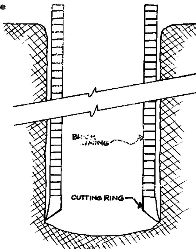
FIG. 8-14. BRICK LINING SUNK ON A CUTTING RING
