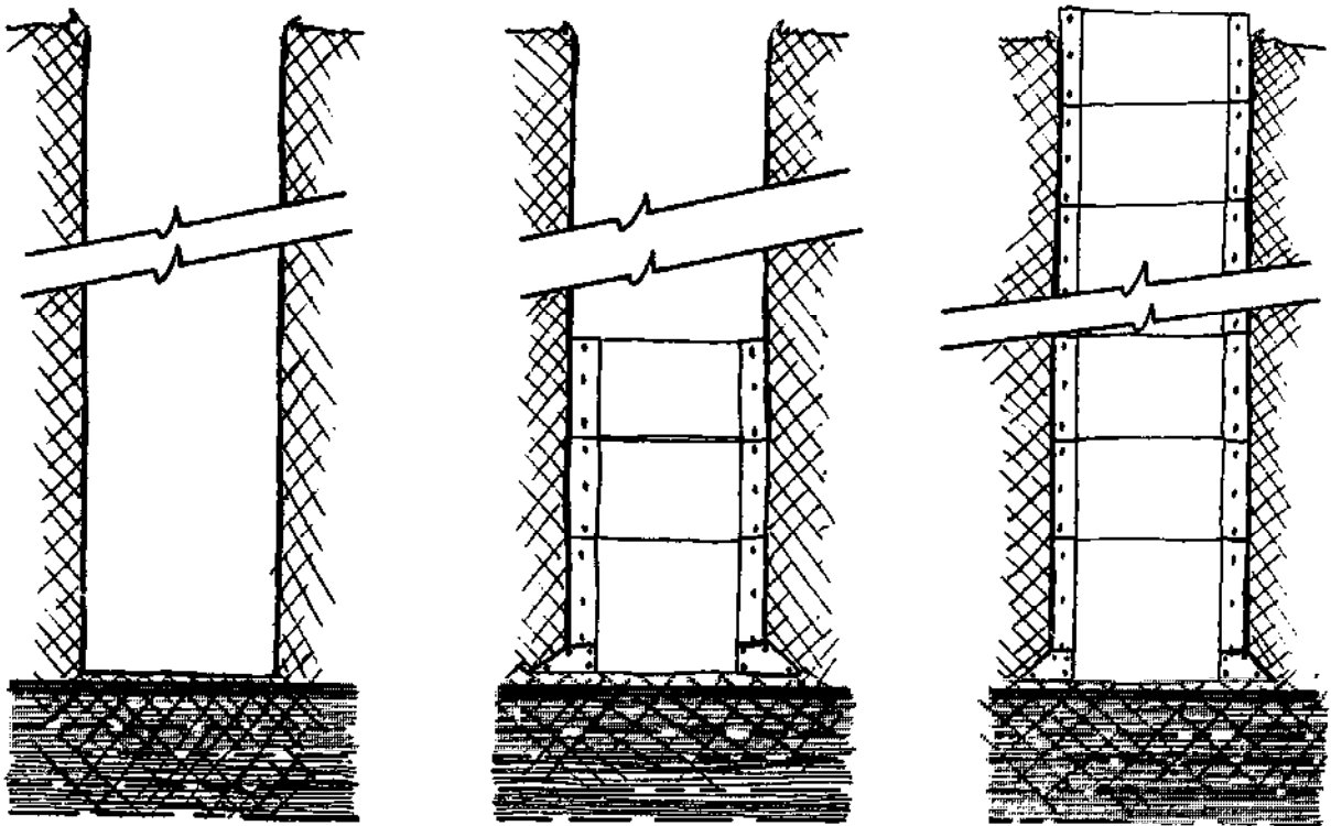
FIG. 8-9. LINING RINGS LOWERED INTO PLACE ON ANCHORING CURB
