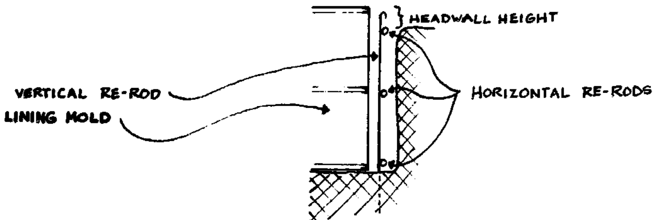
FIG. 8-3. PLACEMENT OF RE-ROD AND FORM IN HOLE
