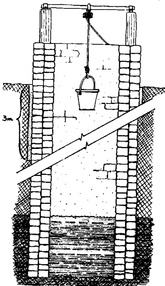
FIG. 8-13. ROCK LINED WELL. 3m. OF CONCRETE OR MORTAR SEAL IS TO PREVENT CONTAMINATION
