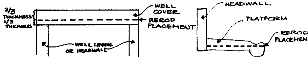
FIG. IV-3. REINFORCING ROD PLACEMENT (ALSO SEE FIGS. 8-3 AND 8-5 FOR REROD PLACEMENT IN LINING)
