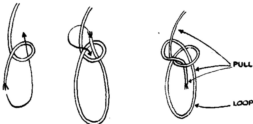
FIG.5-9. BOWLINE
