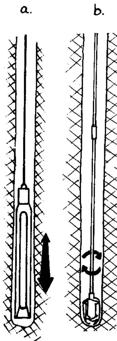
FIG. 10-2. DRILLING MOTIONS
