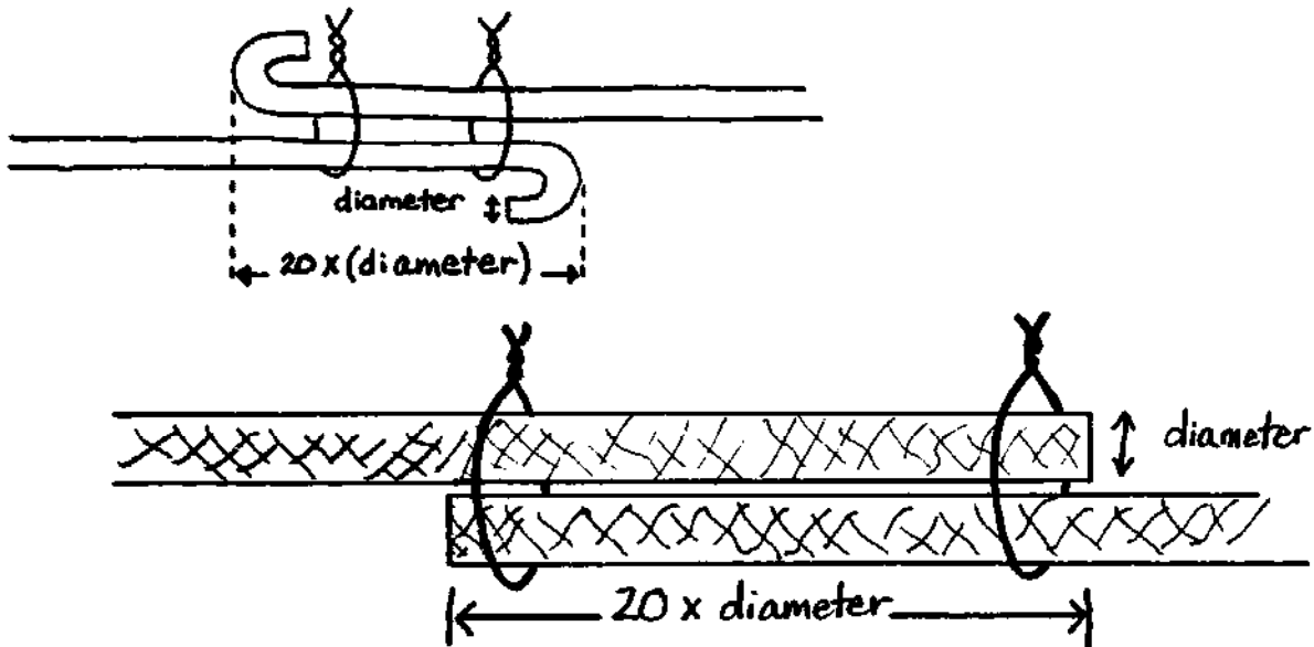
FIG. IV-4. REBAR OVERLAP
