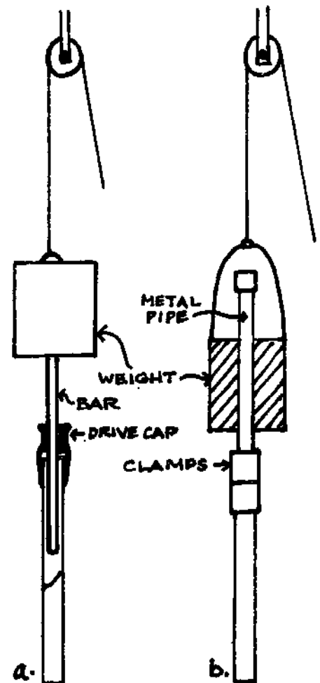
FIG. 14-8. HEAVY DRIVING WEIGHTS
