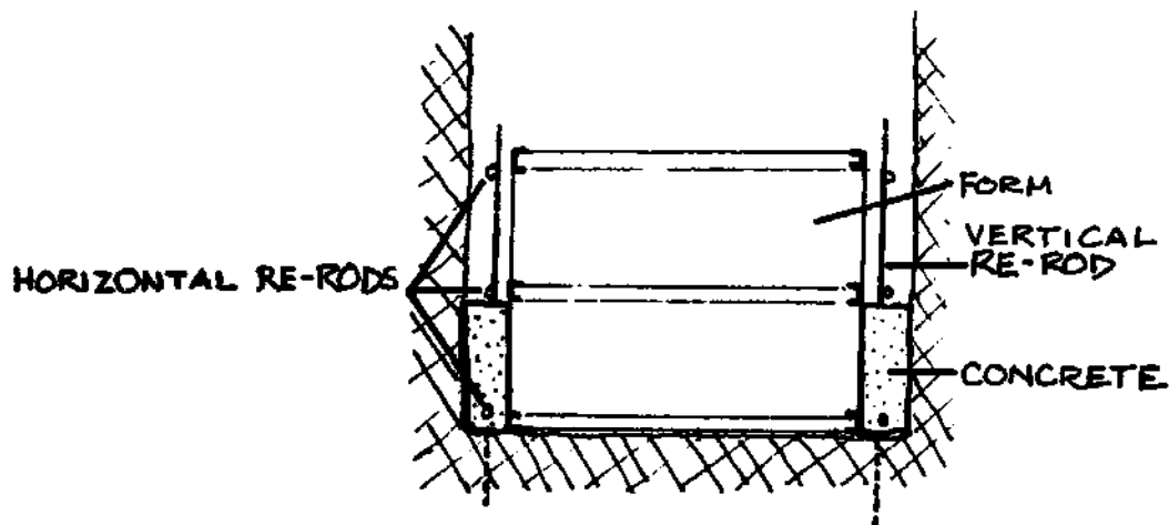
FIG. IV - 2. INTERIOR LINING FORM
