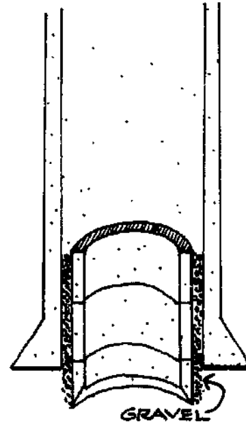
FIG. 9-5. GRAVEL USED TO GUIDE SINKING RINGS
