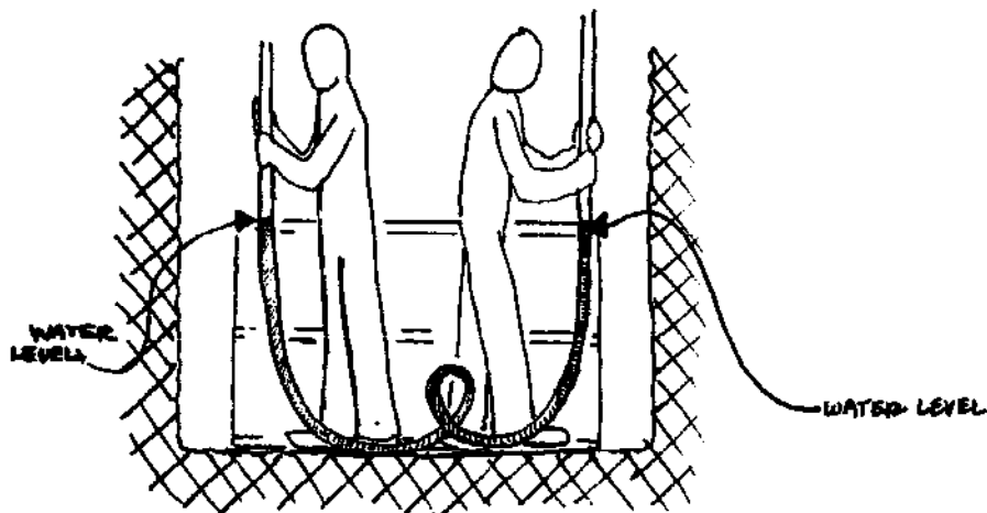
FIG. V-4. CLEAR HOSE AND WATER USED AS LEVEL
