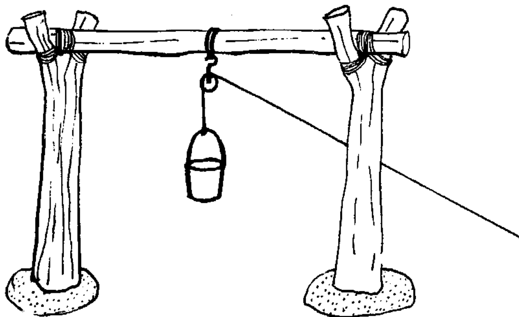
FIG.5-4. WOOD LOWERING SUPPORTS
