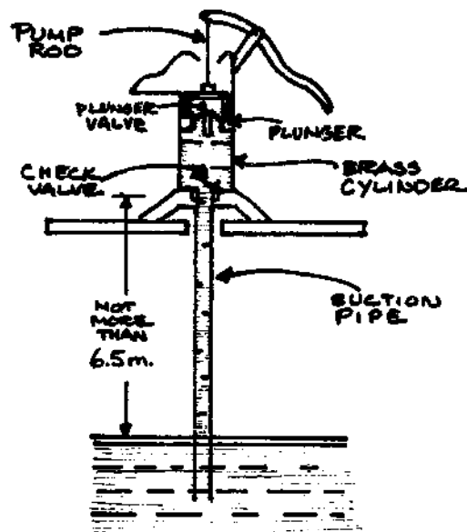
FIG. VII - 2. SHALLOW WELL LIFT PUMP
