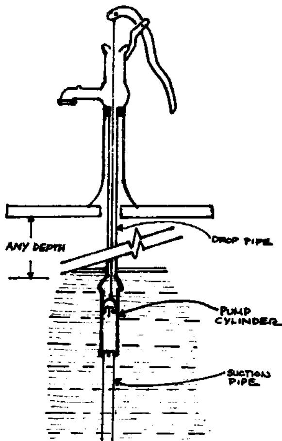
FIG. VII - 3. DEEP WELL LIFT PUMP
