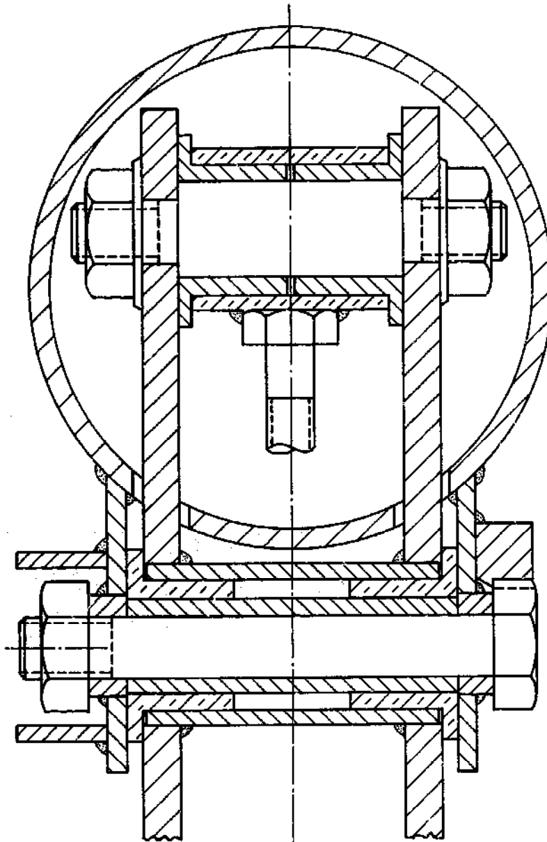
Figure 3-6 General Arrangement of Fulcrum and Rod Hanger Assembly for Acetal Bearings Modified Maidev Handpump — Afridev
