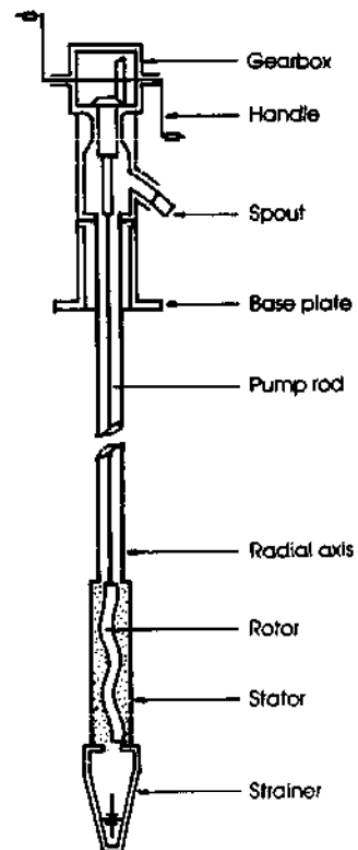
Fig. 10. Model Deep-well Rotary Pump
