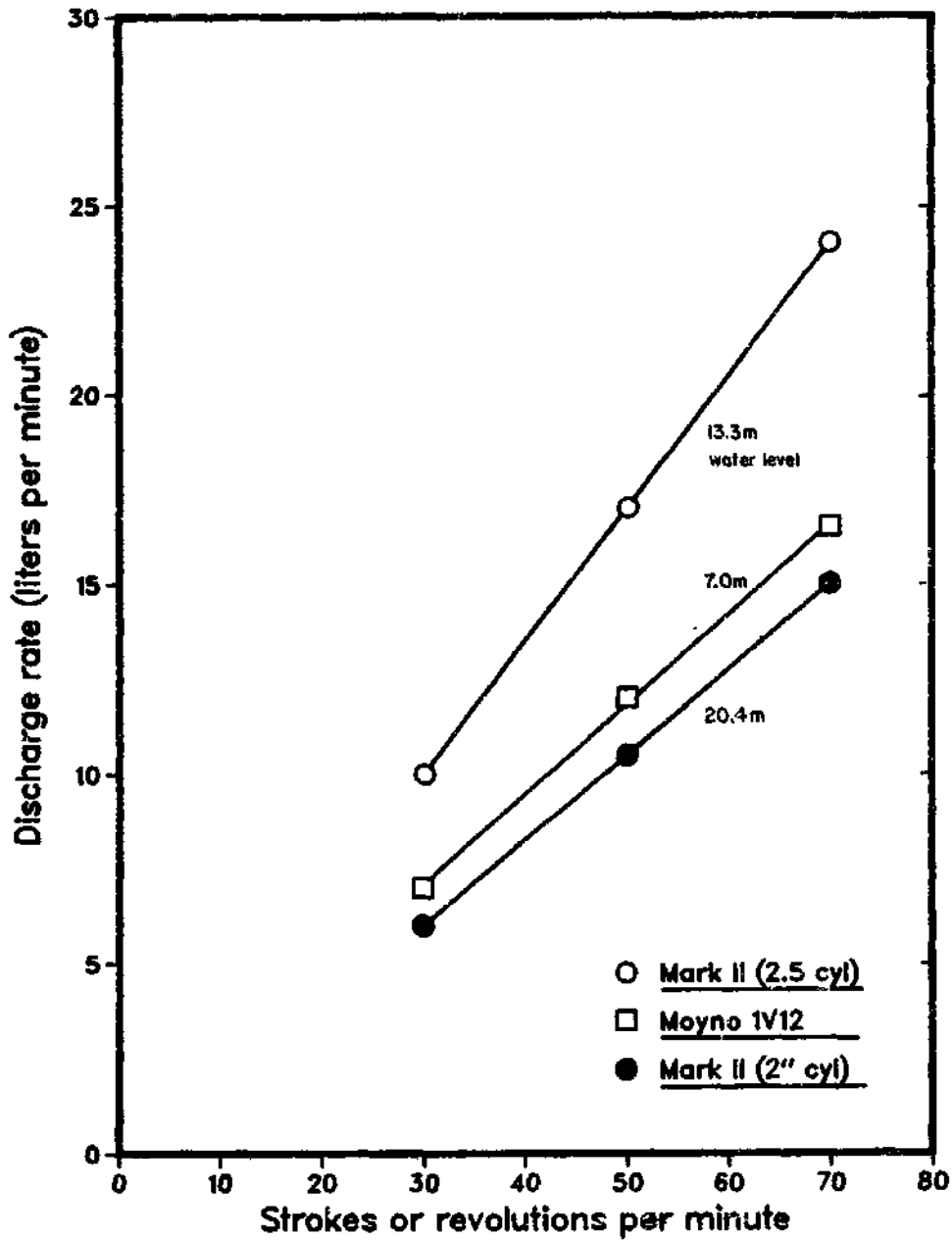
FIGURE 3-9 DISCHARGE RATE VS. HANDLE SPEED INDIA MARK II AND MOYNO PUMPS Ghana Field Trial Area
