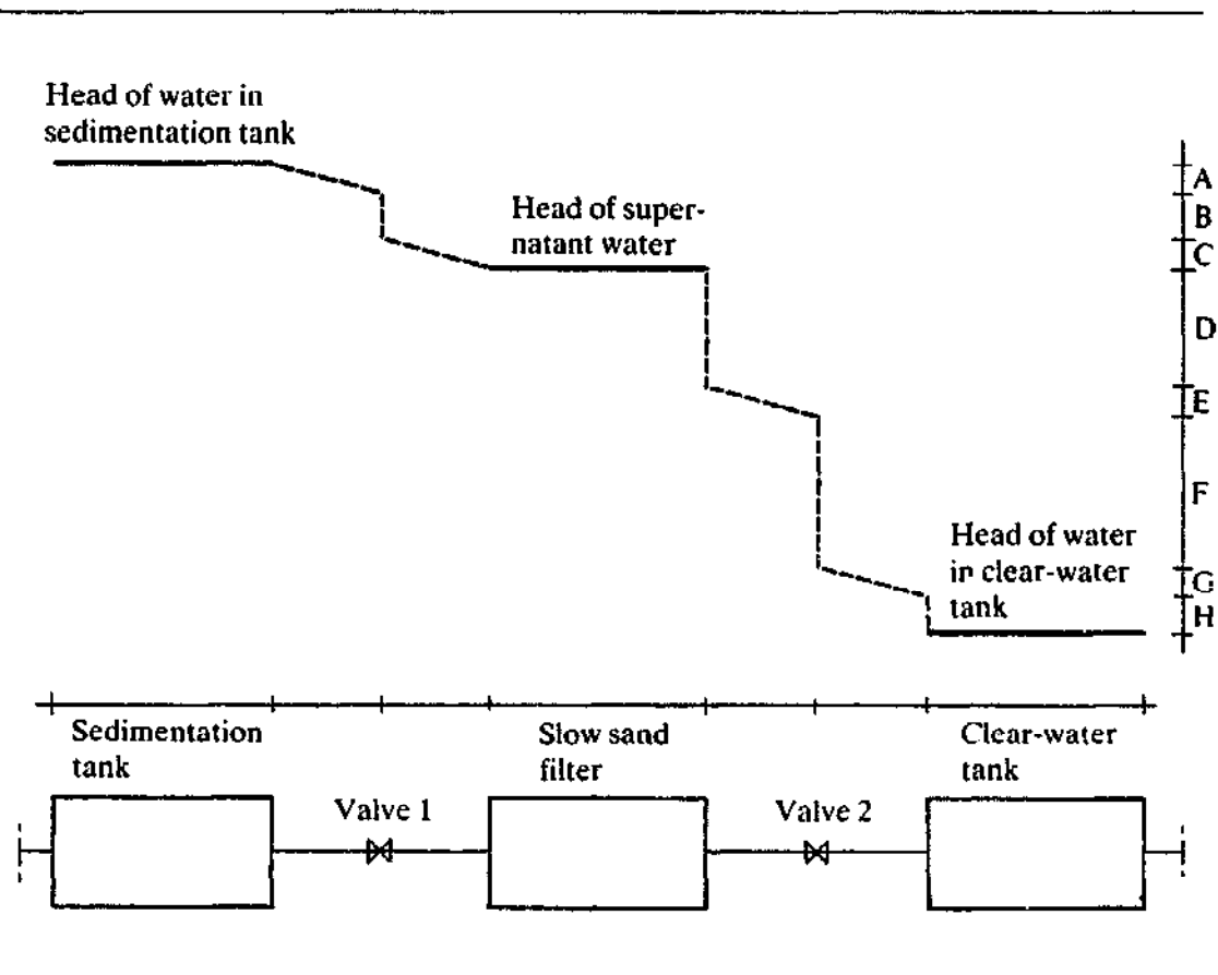
Figure 7.21: Hydraulic gradient line in a slow sand filtration plant (gravity flow)
