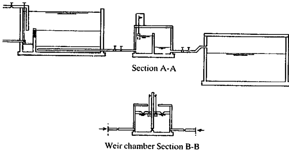
Figure 8.3: Design features of design example III
