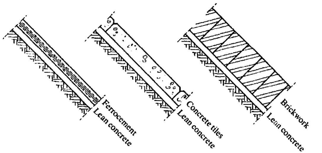
Figure 7.12: Various linings for sloping wall filters
