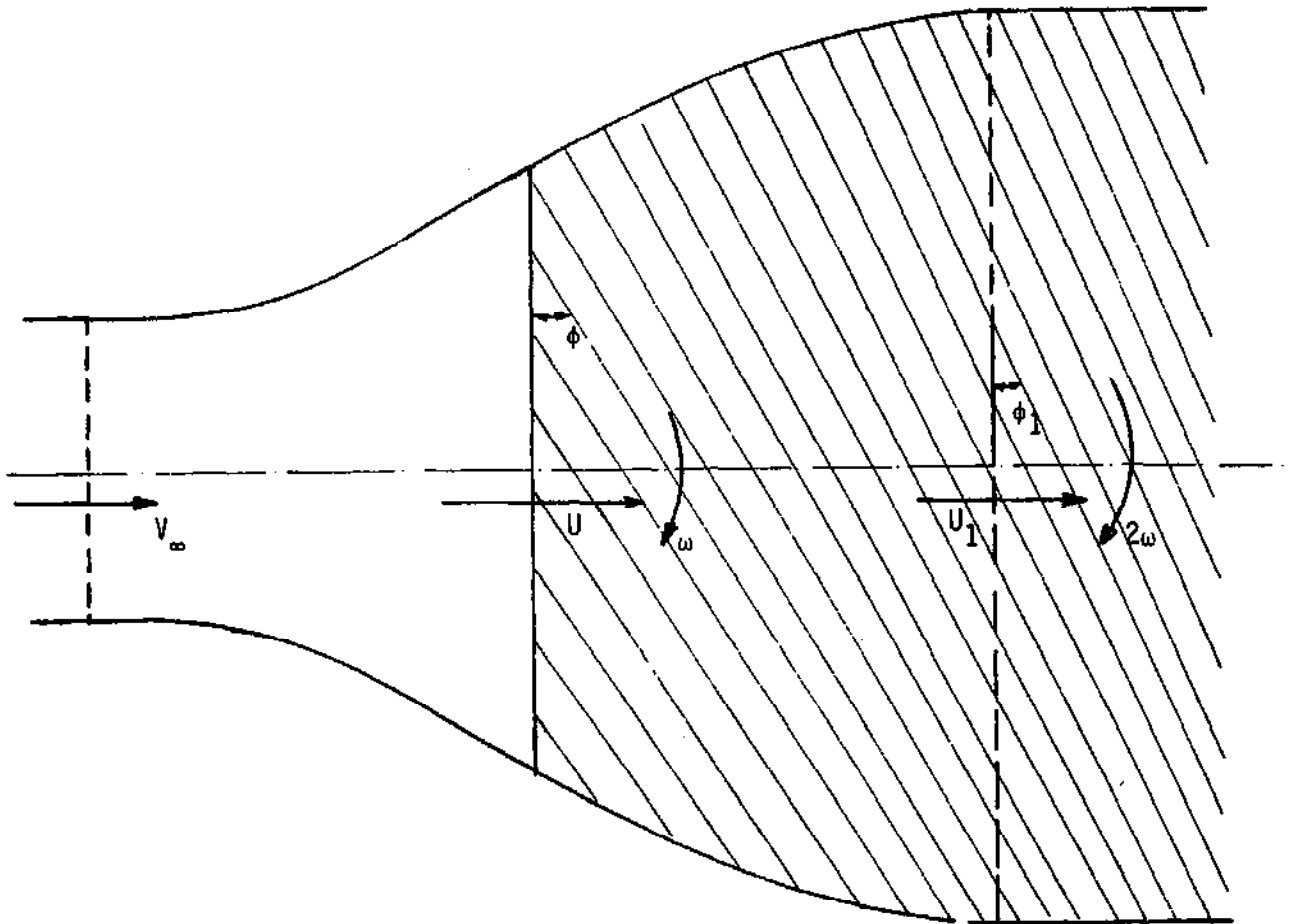
fig. 1.9b. Vortex sheets of heavy loaded multy bladed propeller.
