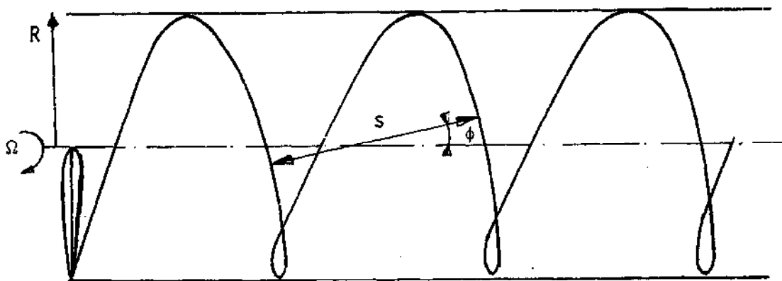
Fig. 1.8.: Vortex sheet of lightly loaded one bladed propeller.
