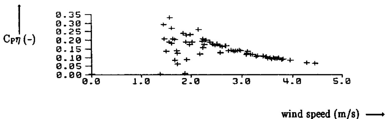
Figure 4.3. Example of overall windpump performance factor curve.
