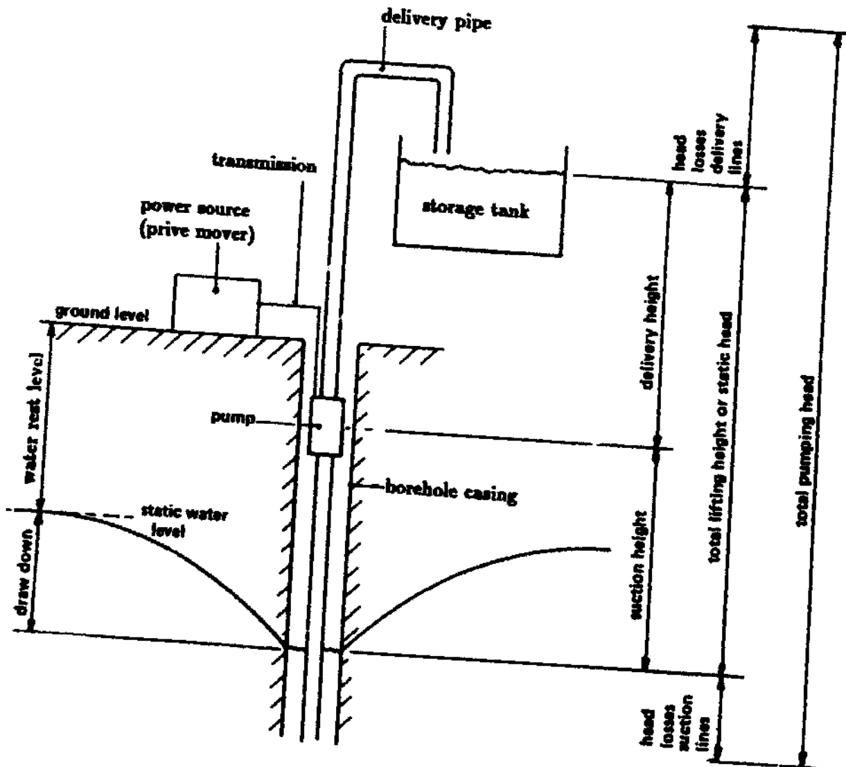
Figure 1.3.b. Composition of total pumping head.
