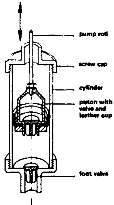
Components of a screw cap pump
