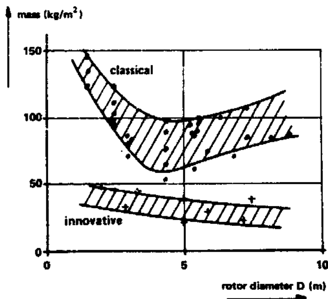
Figure 5.2. Trends in specific mass ( kg/m^2 rotor area) of classical multiblade and modern design wind pumps. Note: values have not been corrected for tower height and pumping depth, but the trend seems sufficiently clear (reference 27).
