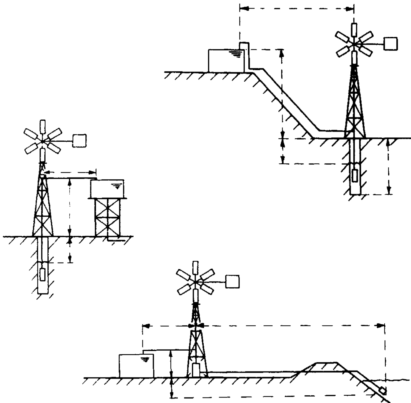
Figure P.1. Examples of layout of wind pumping systems. Indicate distances and heights for tender document.
