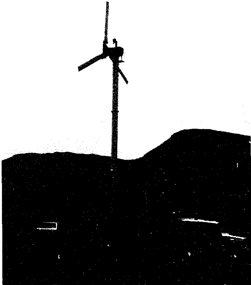
Wind electric pumping system (WEPS) on Cape Verde. A Lagerwey wind turbine of 10.6 m rotor diameter is installed on an 'achada', well exposed to the wind, and drives an electric deep-well pump in the valley. Note the hydraulic jack at the tower base for erection without the need for a crane.
