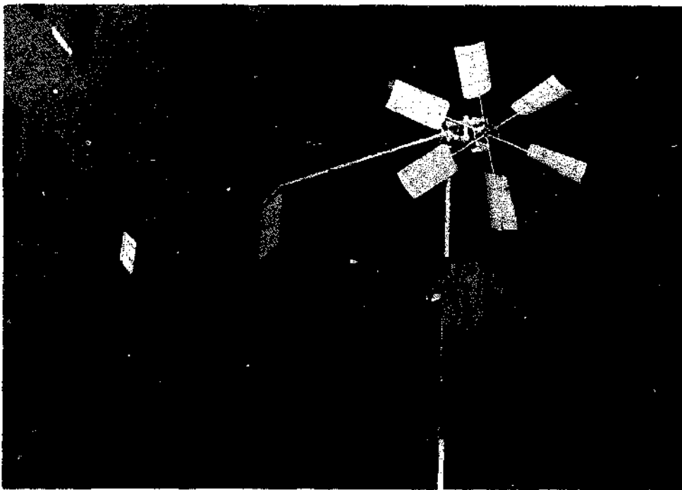
Testing a full scale 2-m diameter wind pump of CWD in the 12x16 m wind tunnel of the Chinese Aerodynamic Research and Development Center (CARD), Mianyang. Note the spar construction of the rotor and the small hinged side vane as part of the safety and control system.
