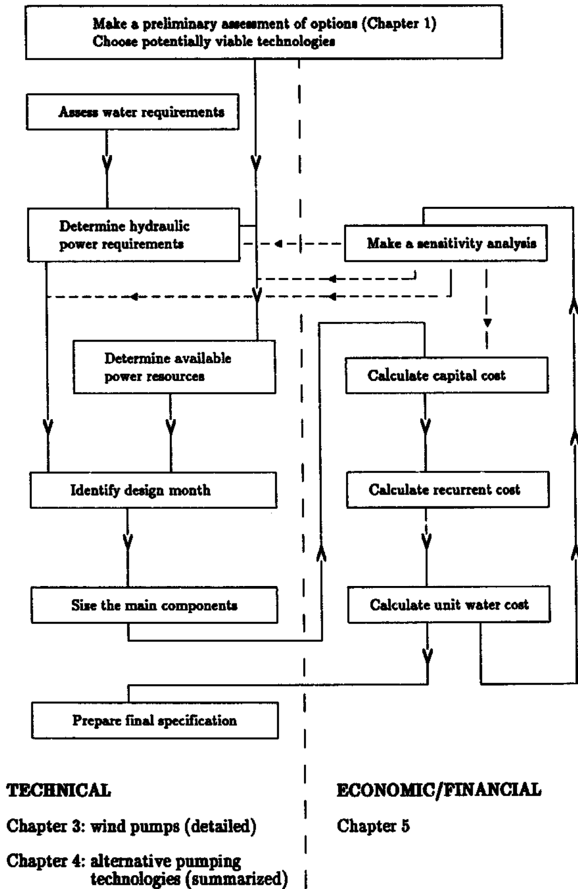
Figure 3.1. Steps to be taken for evaluation and design of pumping installations.
