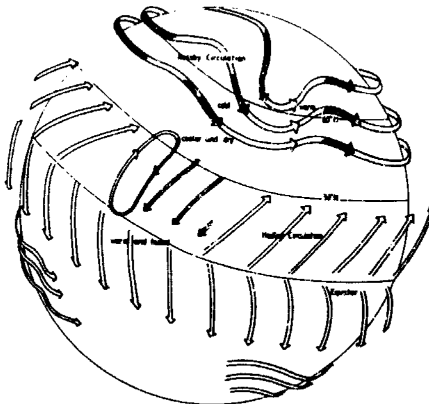
Figure A.1. Schematic picture of the general circulation of air around the globe. North and South of 30^{\circ} N and 30^{\circ} S, respectively, a westerly circulation prevails, while in the tropics one finds NE and SE trade winds (reference 7).
