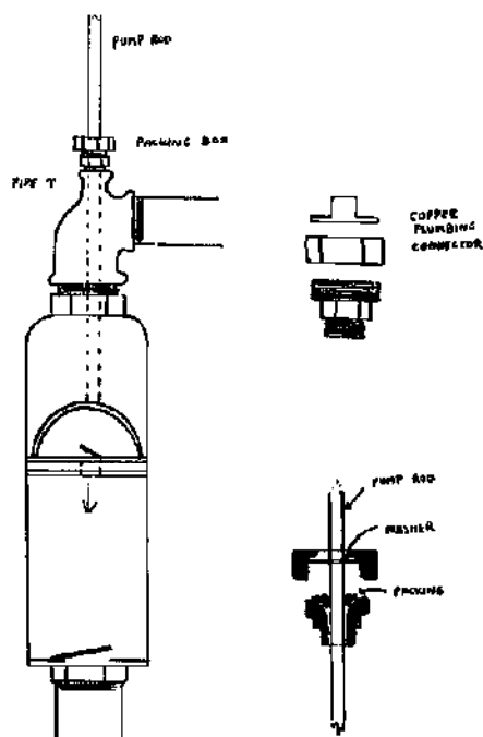
Figure 5 Inexpensive packing box for piston pump.
