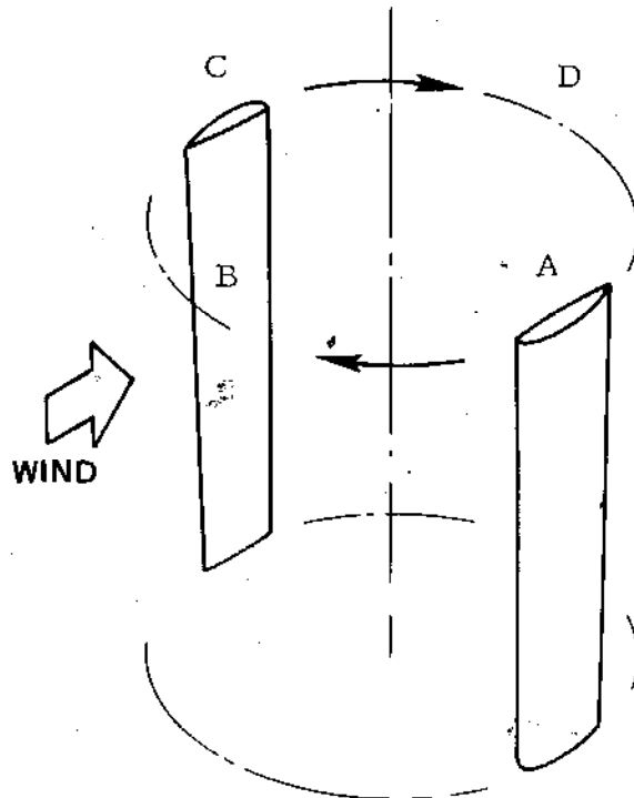
Figure 12 Hybrid Concept
