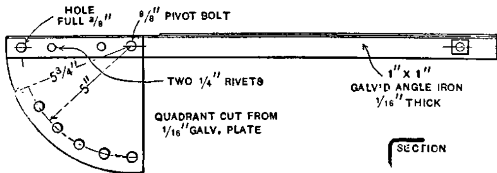
FIG. 37.—Elevation and Plan of Tail Regulator.
